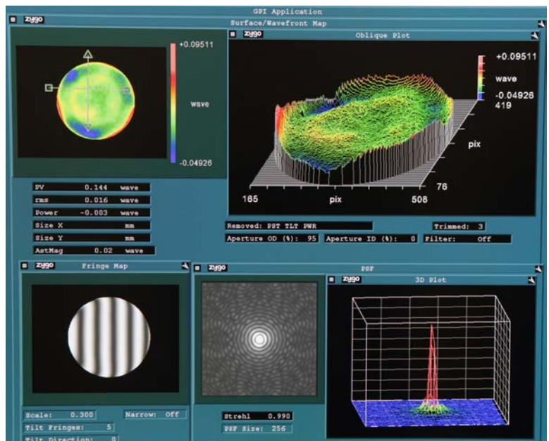
Sample screenshot taken during our Zygo Interferometer testing. Your SVX130T telescope came with a printout just like this but it is of its own test to verify its high optical standard.
