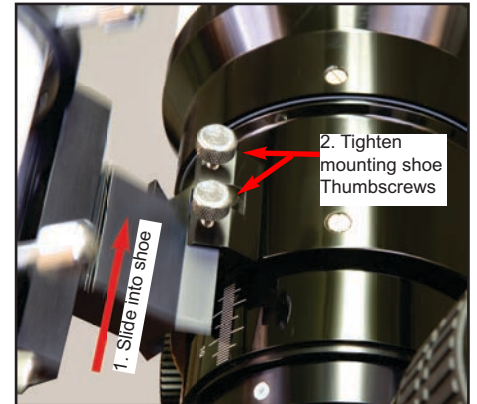
Mounting finderscope and rings
