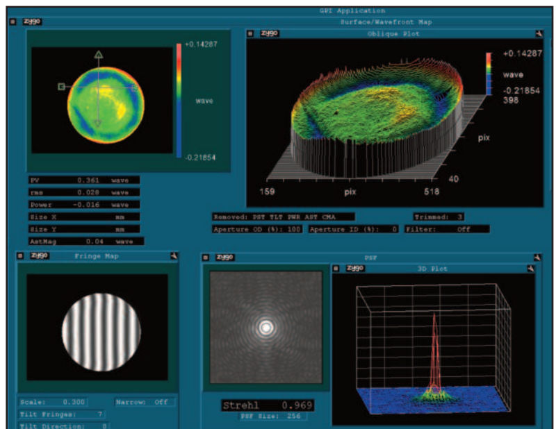
Sample screenshot taken during our Zygo Interferometer testing. Your SVX102T and SVX102T-R telescope came with a printout just like this but it is of its own test to verify its high optical standard.
